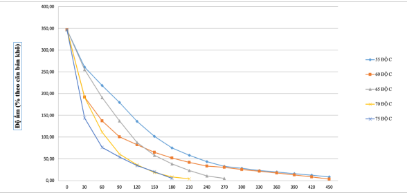
Fig. 3: Drying curves at different temperatures
