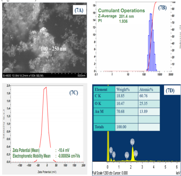
Fig. 7: SEM (7A), DLS (7B), Zeta (7C), and EDX (7D) of DH-AuNPs
